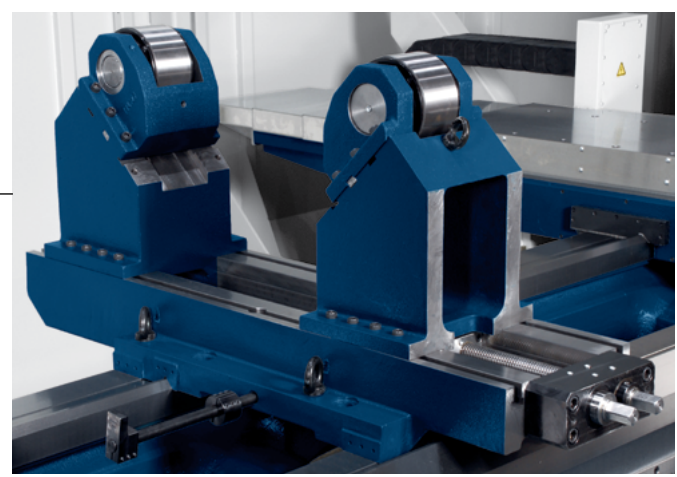
Steady rest C type (optional) Table rest (optional) Equipped with rollers and manual diameter adjustment. It has a drag system via longitudinal saddle for its positioning.
